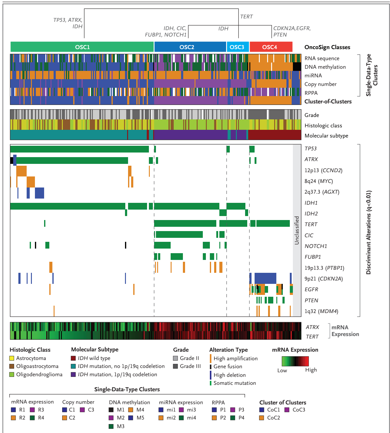
Figure 3. OncoSign Analysis.
