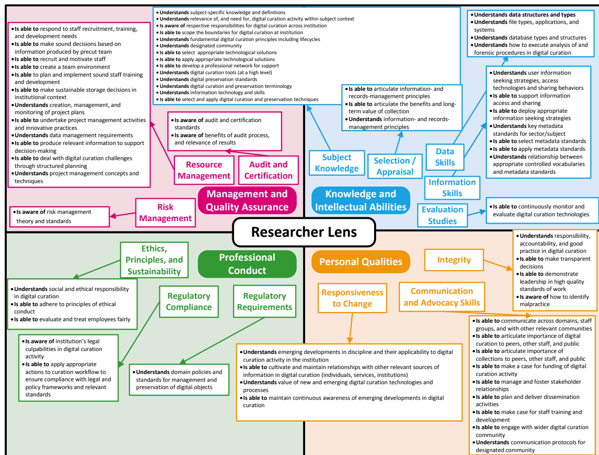
Figure 12: Researcher Lens
