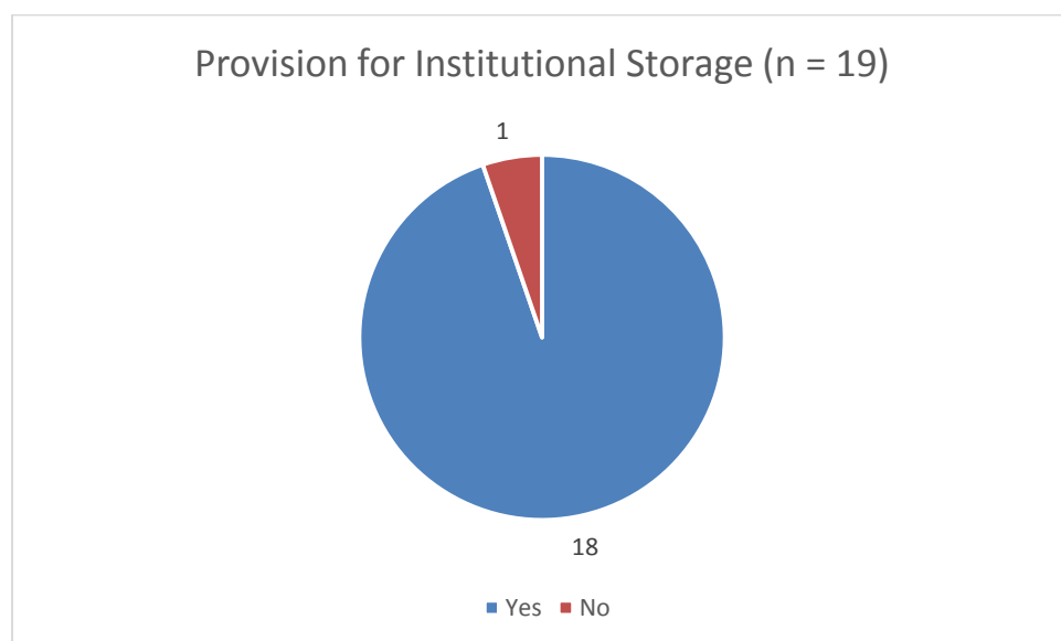
Figure 8: Institutional Storage
