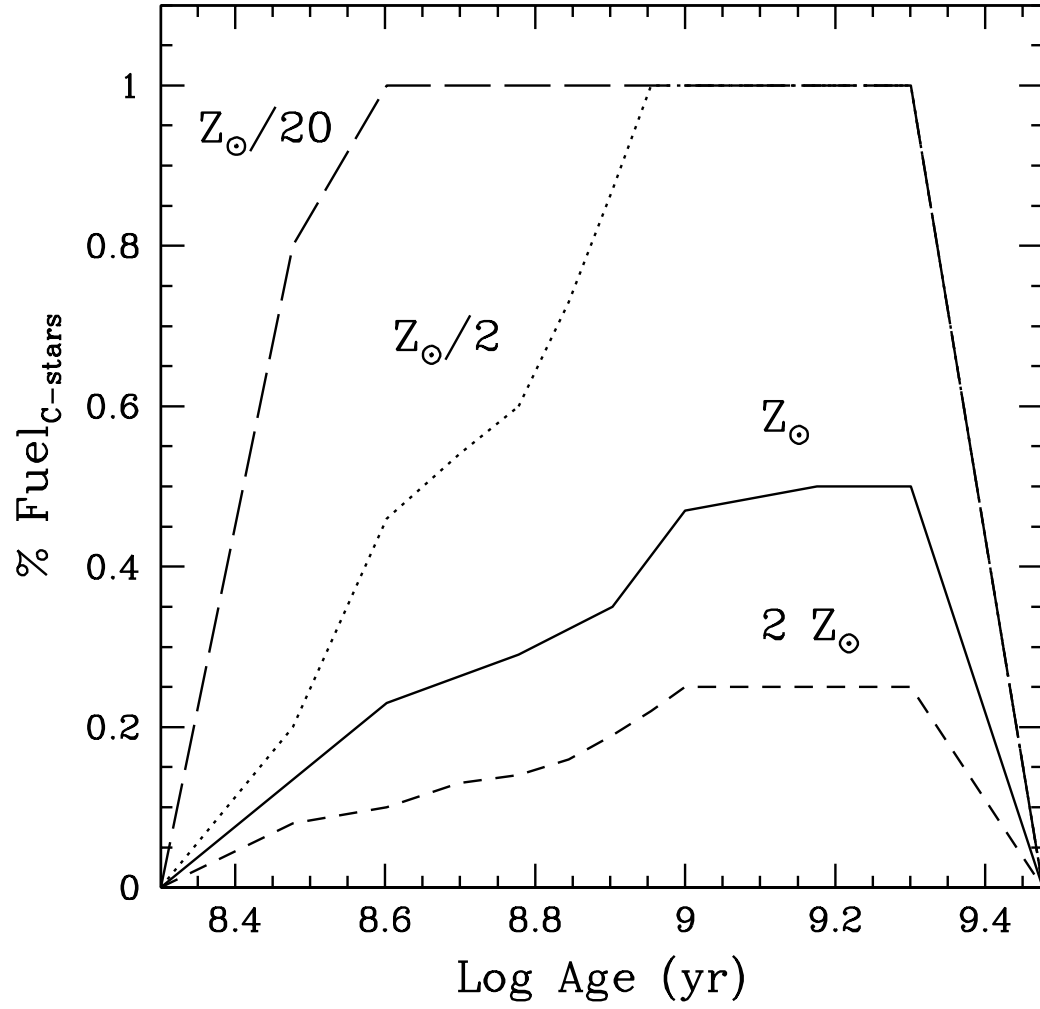
Figure 3.6 - Percentage of TP-AGB fuel spent in C-stars as a function of metallicity in the M05 SPS models. Note the strong metallicity dependence, and the increase with age for each metallicity until \sim 2 Gyr. (Figure 12 from M05, reproduced with permission.)
