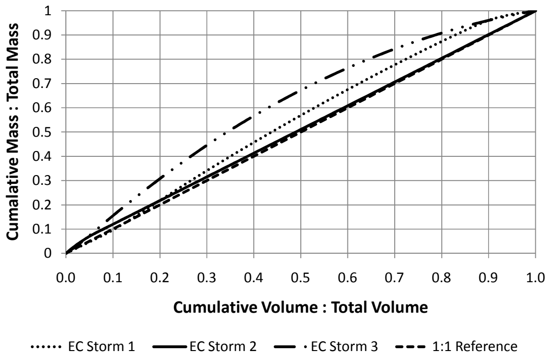
Figure 16: Individual EC M/V curves, Meeting of the Water Creek (MWC).
