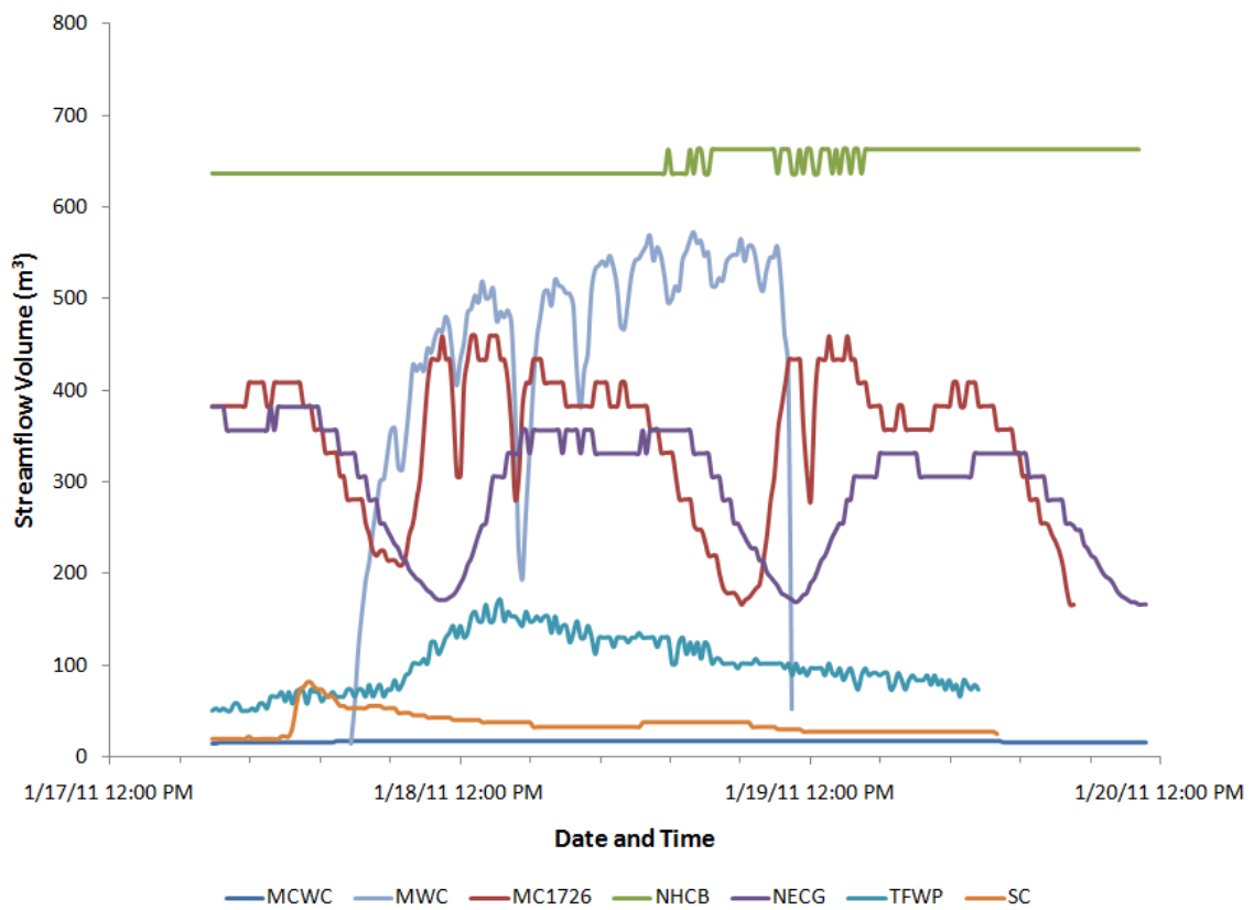
Figure 10: Storm event 3 hydrographs at all gauged creeks.
