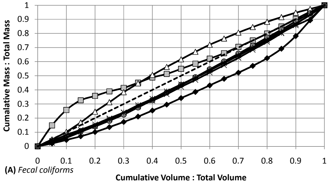
Figure 2: Average mass to volume ( M/V ) curves for (A) FC and (B) EC at each gauged creek site.
