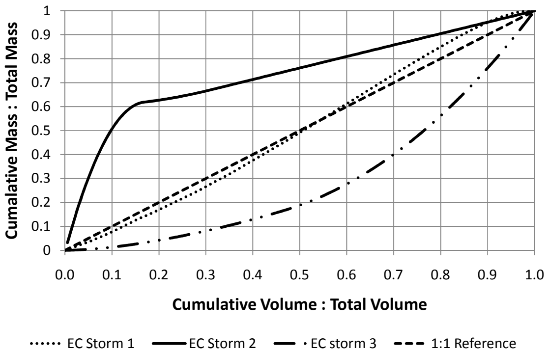
Figure 14: Individual EC M/V curves, Morgan Creek at NC-54 West (MCWC).
