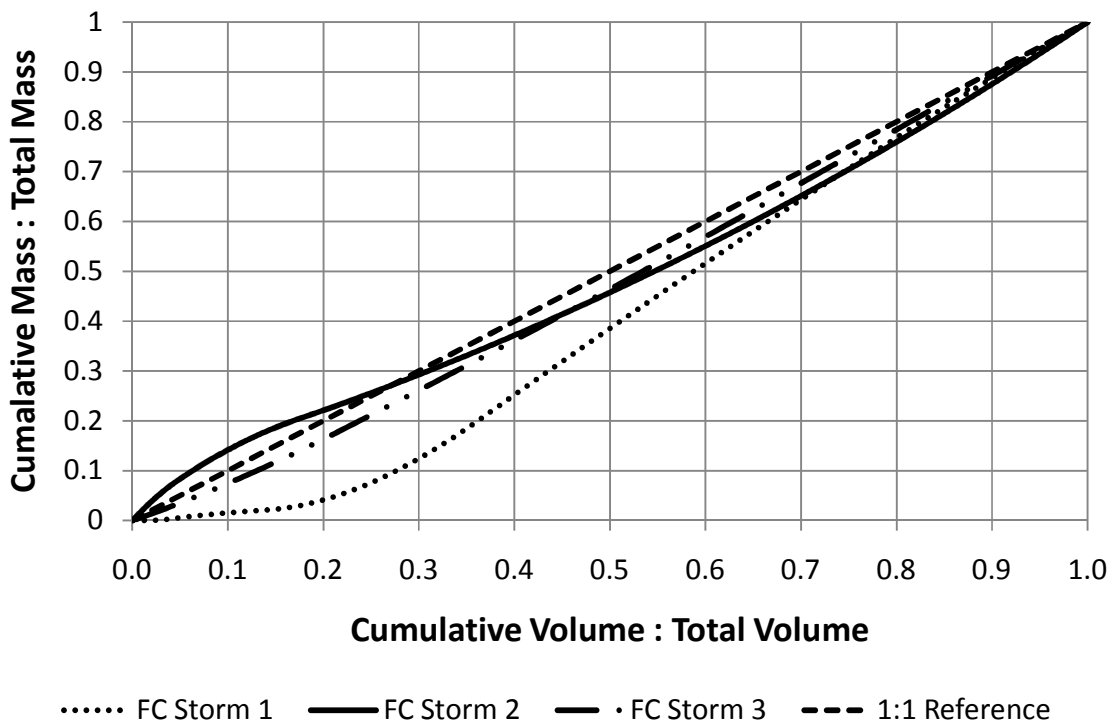
Figure 19: Individual FC M/V curves, New Hope Creek at Blands (NHCB).
