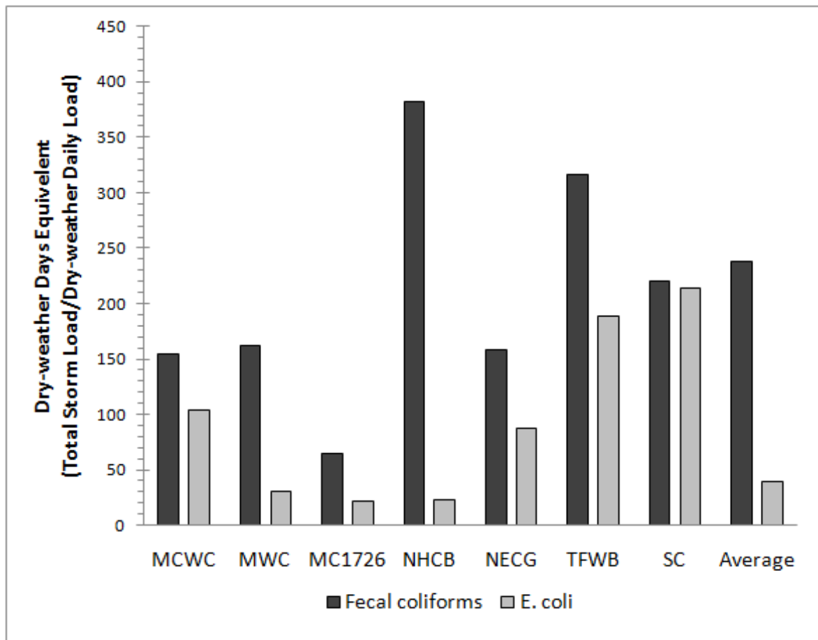
Figure 12: Storm event loading patterns at all gauged creek sites and all creek sites combined.
