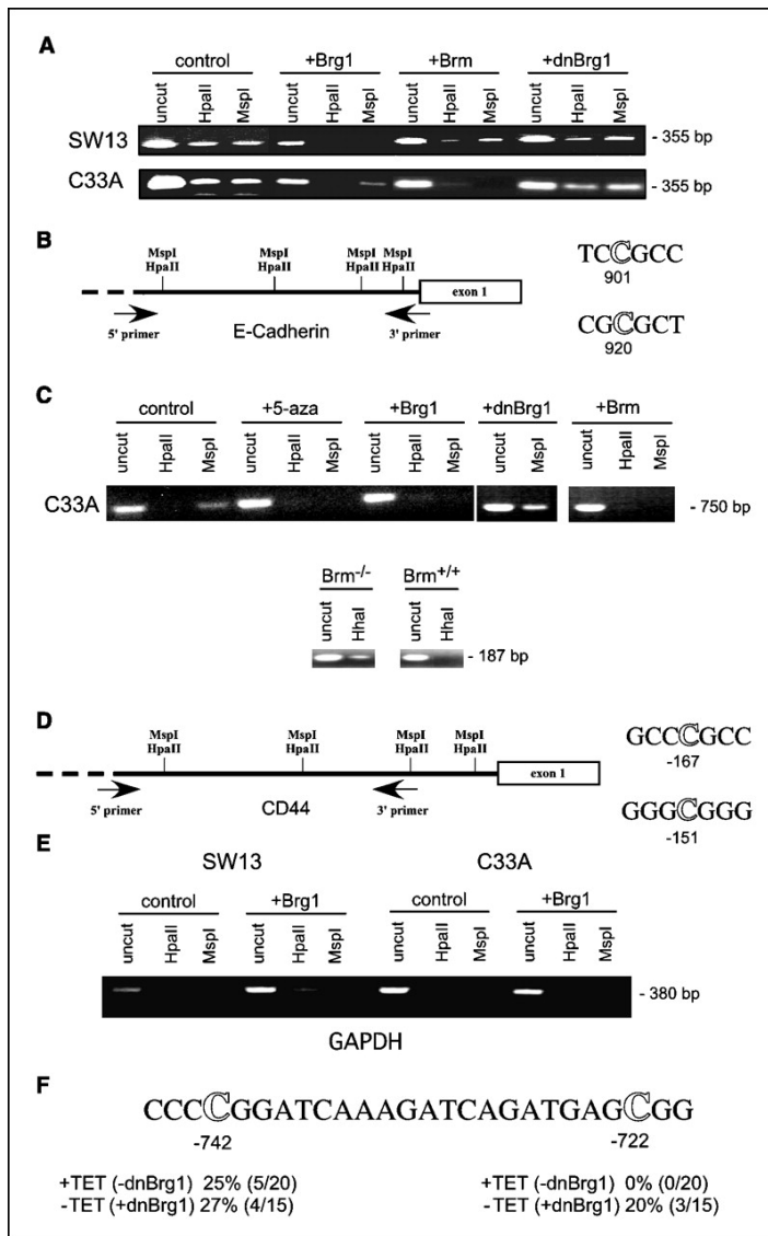
Figure 3.3: Brg1 and Brm cause loss of DNA methylation in the 5' untranslated regions of CD44 and E-cadherin. A , SW13 and C33A cells were transfected with Brg1, Brm, mutant Brg1 (dnBrg1), or an empty vector. DNA was isolated, incubated with methylation-sensitive restriction enzymes as indicated, and amplified using the primers shown in ( B ). B , altered methylation was verified by bisulfite sequencing, which demonstrated a loss of methylation in 100% of clones sequenced at cytosines 901 and 920. These sequences have previously been reported to be hypermethylated in some cancer cell lines. C , loss of DNA methylation was also observed in the CD44 promoter following treatment of C33A cells with 5-aza (as a positive control) or transfection with Brg1 or Brm but not mutant Brg1 ( top ). D , primers used to amplify enzyme-treated DNA. We also observed consistent loss of DNA methylation in the
