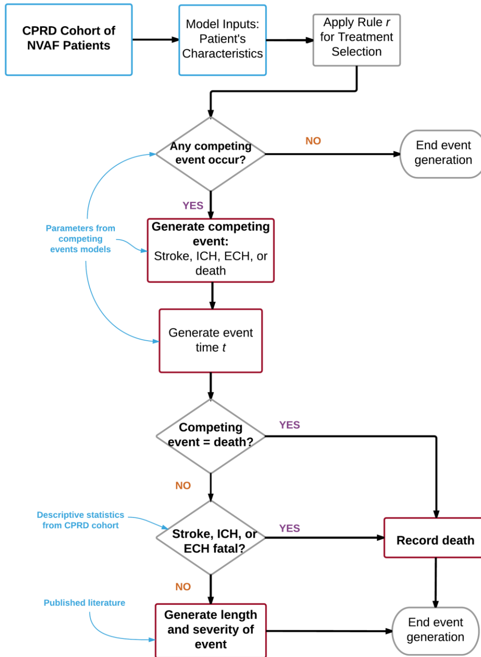
Figure 5.1 Framework for Individual-Based Simulation
