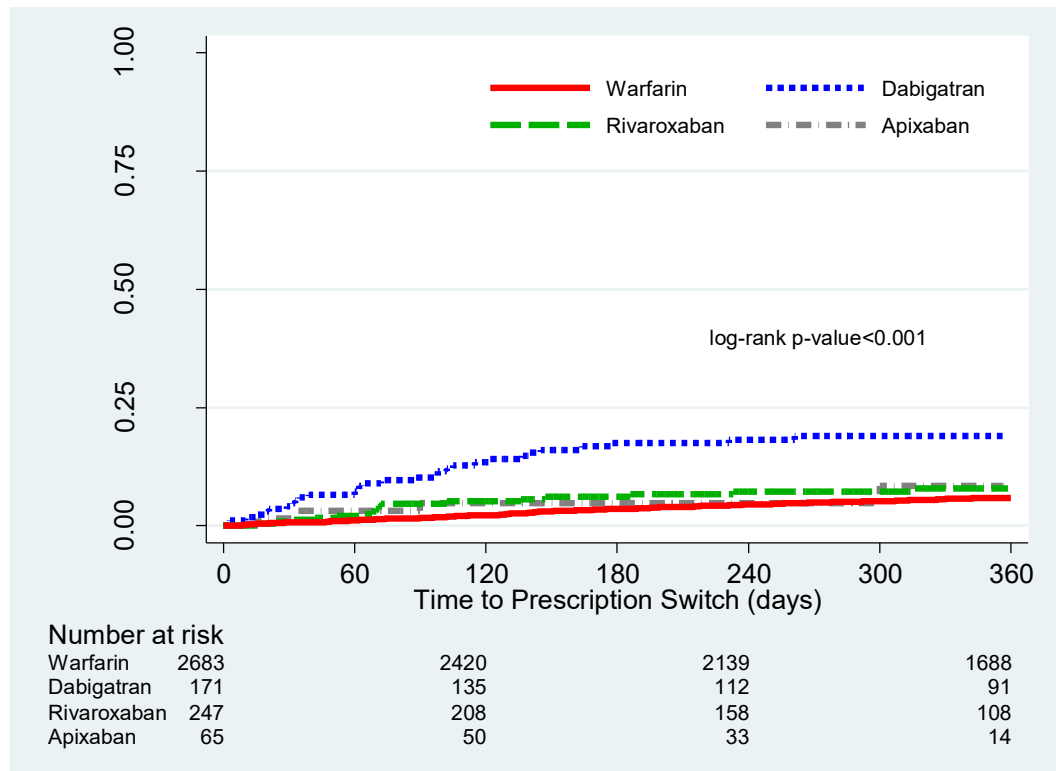
Figure 3.5 Kaplan-Meier Estimate of the Cumulative Incidence of an OAC Switch - Patients Diagnosed with NVAf in the Years 2013-2014
