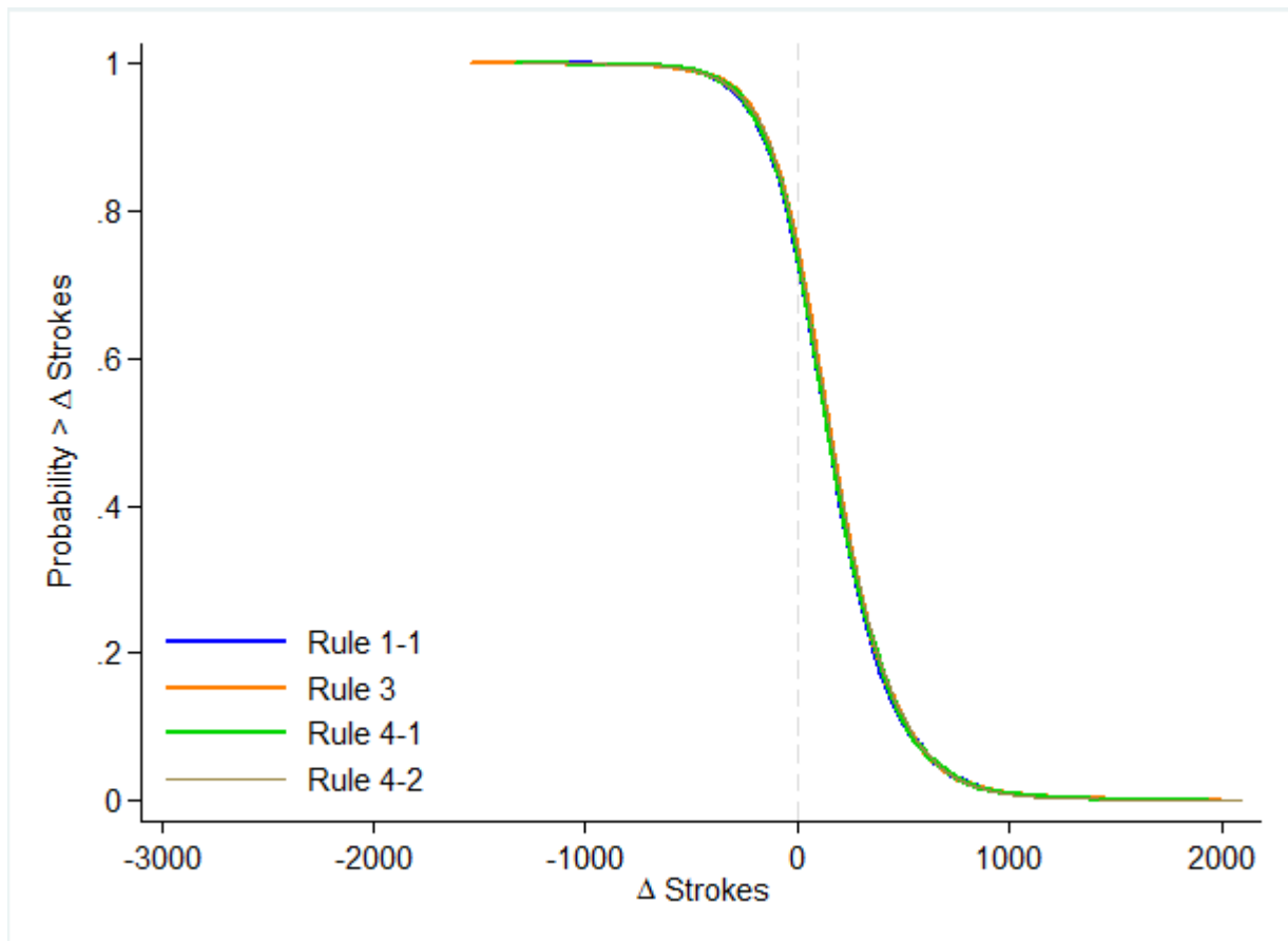
Supplemental Figure 8. Complement Cumulative Distribution Plot of Strokes Avoided vs. Current Treatment Patterns for Four Superior Treatment Selection Rules
