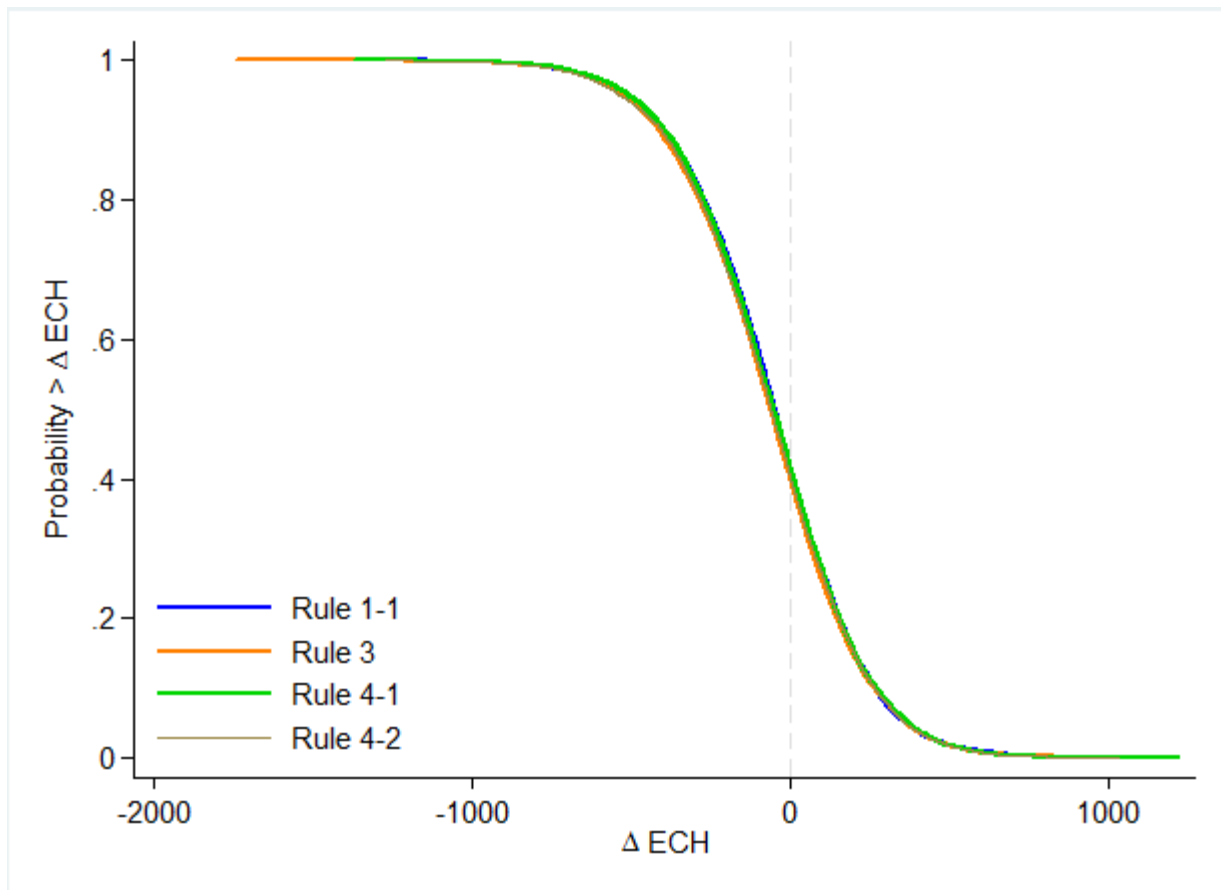
Supplemental Figure 10. Complement Cumulative Distribution Plot of Extracranial Hemorrhages Avoided vs. Current Treatment Patterns for Four Superior Treatment Selection Rules
