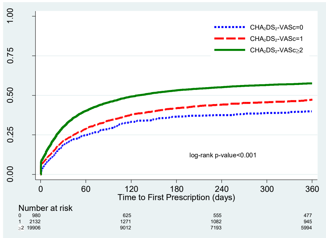
Figure 3.2 Kaplan-Meier Estimate of the Cumulative Incidence Function of First OAC Prescription by CHA 2 DS 2 -VASc Risk Score
