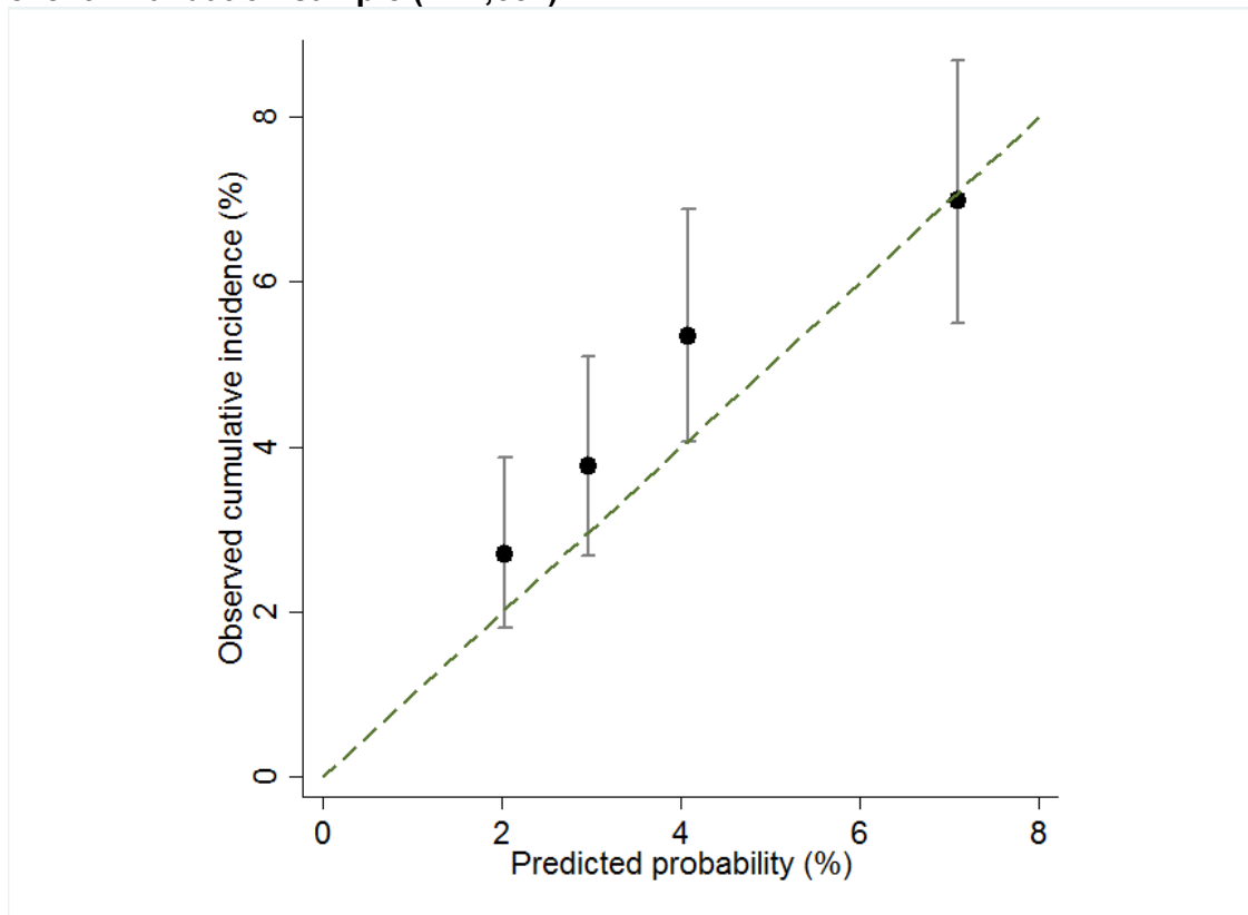
Supplemental Figure 6. Calibration plot for extracranial hemorrhage as a first clinical event – validation sample (N=4,654)
