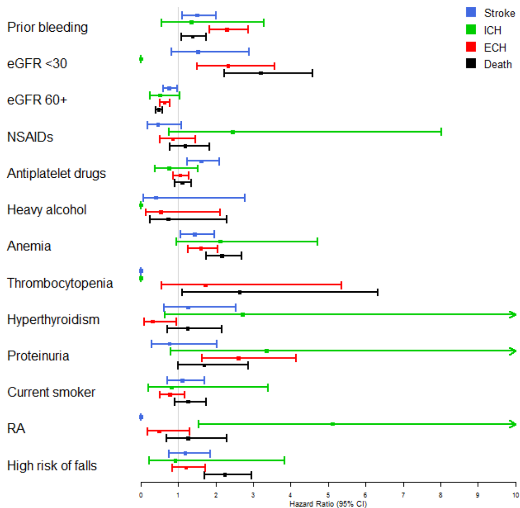
Supplemental Figure 4. Subdistribution hazard ratio (95% CI) of first clinical event by cause for all potential predictors as main effects from Fine-Gray competing risks regression models – development sample (N=10,829)
