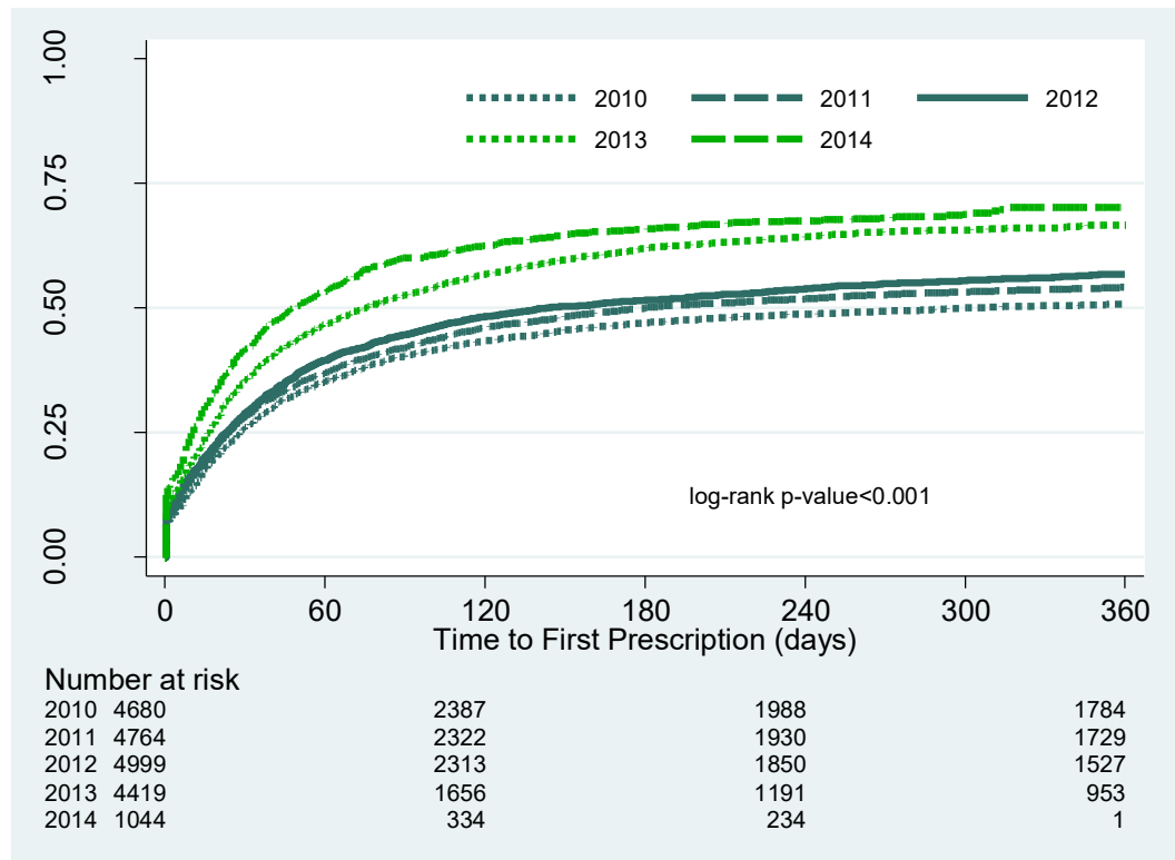
Figure 3.3 Kaplan-Meier Estimate of the Cumulative Incidence of First Prescription for OAC by Year of AF Diagnosis - Patients with \text{CHA}_2\text{DS}_2\text{-VASc} \geq 2
