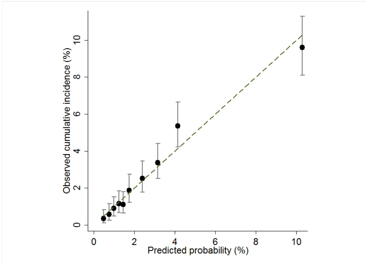
Figure 4.1 Calibration Plot for Stroke as a First Clinical event - Full Study Cohort (N=15,483)
