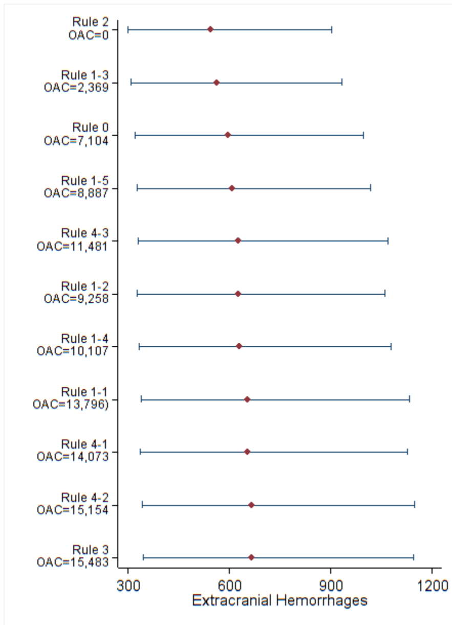
Supplemental Figure 4. Mean and 95% Confidence Interval for Number of Extracranial Hemorrhages (10,000 runs)
