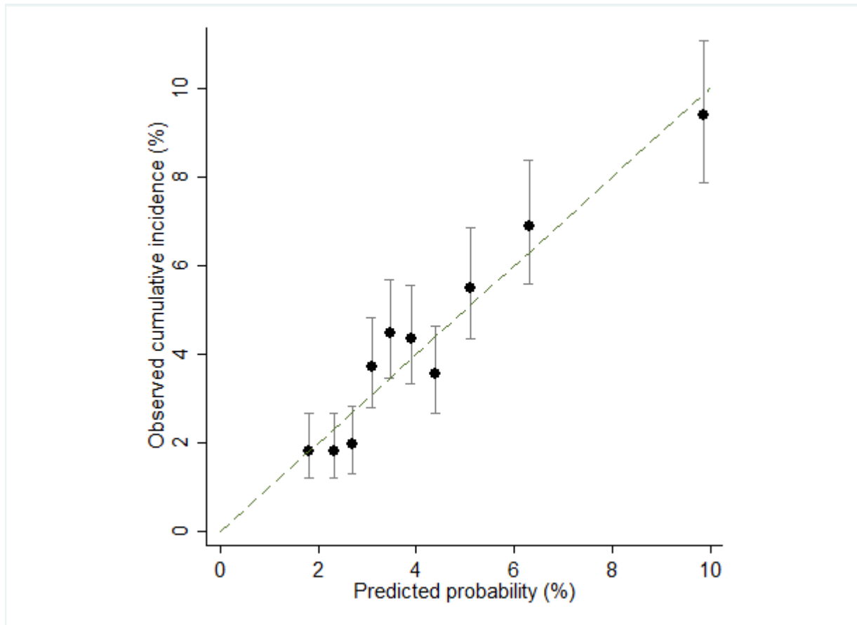
Figure 4.3 Calibration Plot for Extracranial Hemorrhage as a First Clinical Event - Full Study Cohort (N=15,483)
