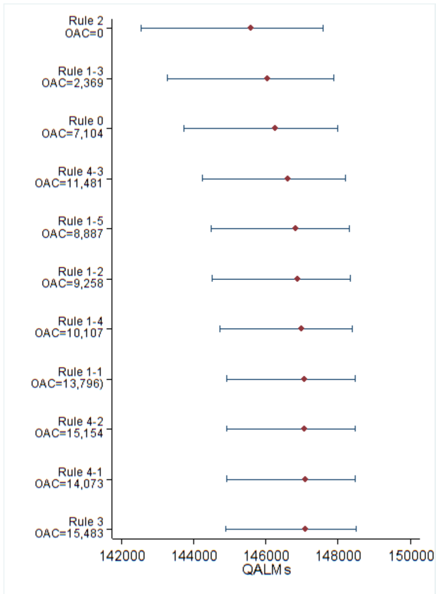
Supplemental Figure 6. Mean and 95% Confidence Interval for Total QALMs (10,000 runs)
