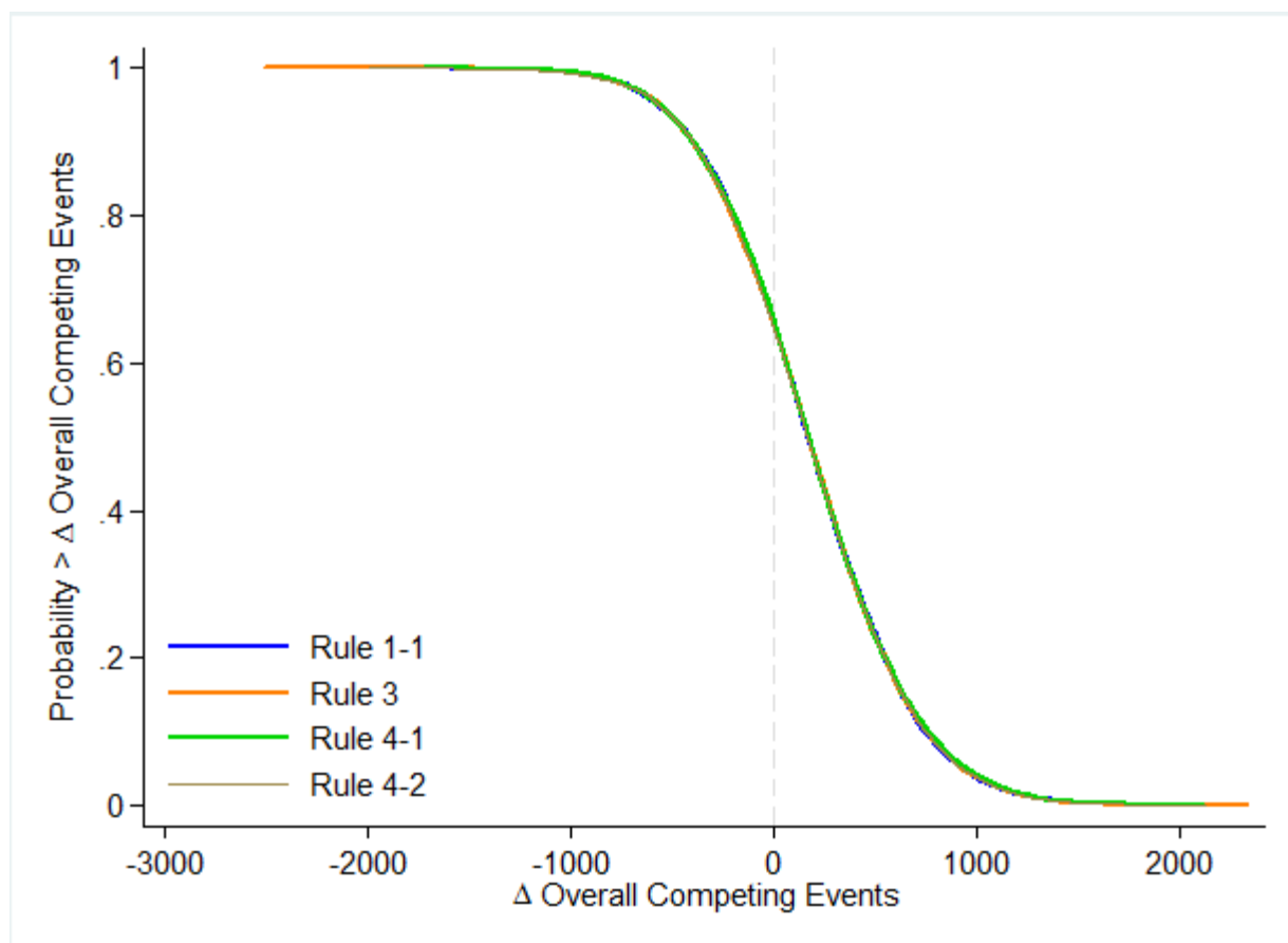
Supplemental Figure 7. Complement Cumulative Distribution Plot of Overall Competing Events Avoided vs. Current Treatment Patterns for Four Superior Treatment Selection Rules
