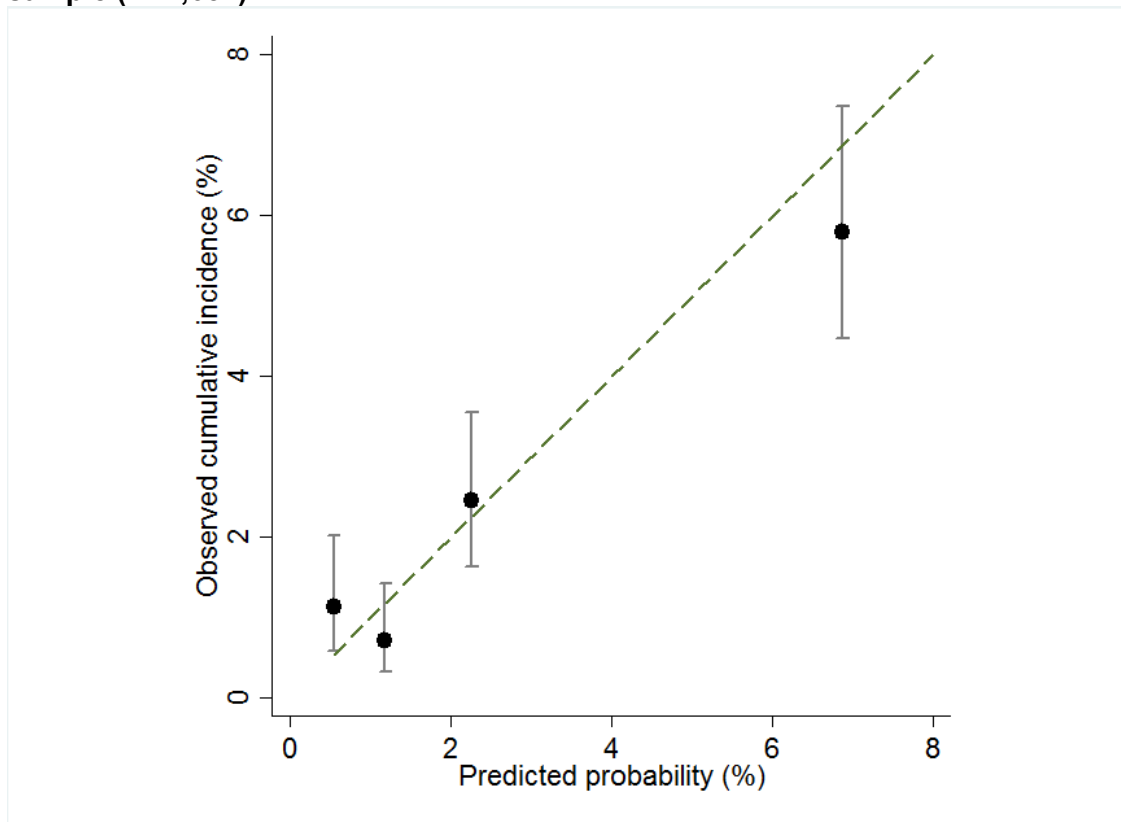
Supplemental Figure 5. Calibration plot for stroke as a first clinical event – validation sample (N=4,654)
