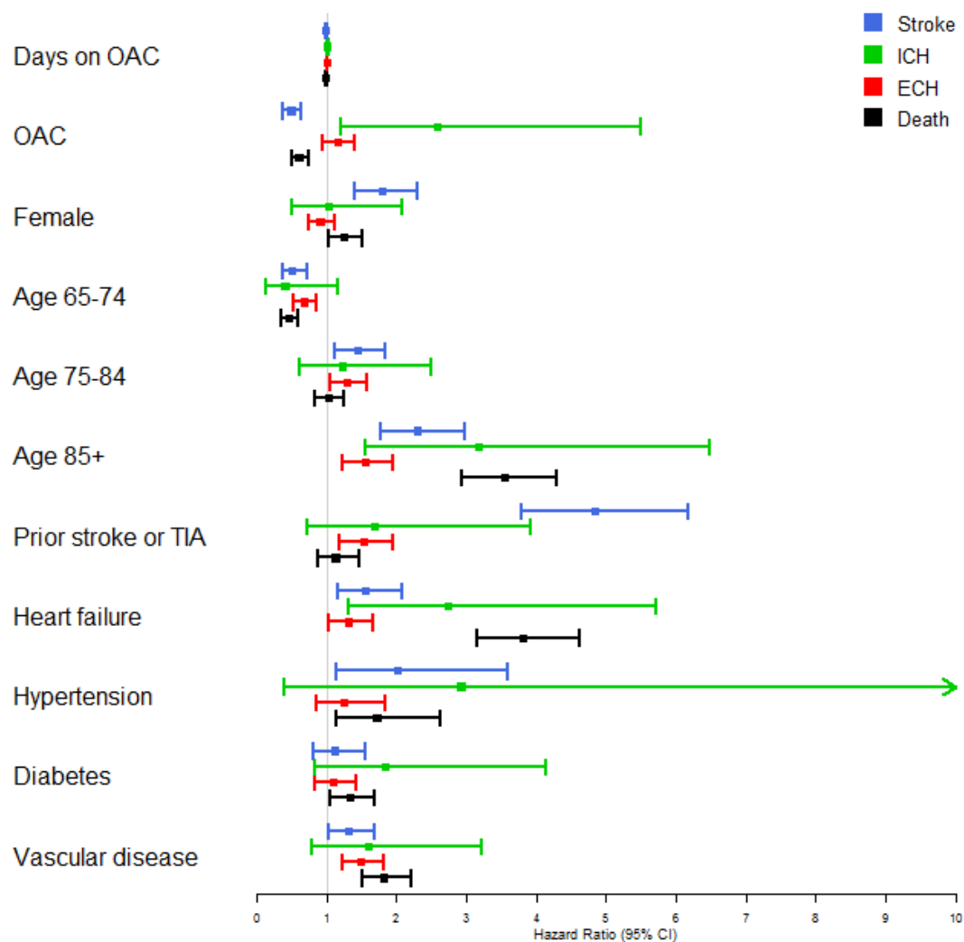
Supplemental Figure 4. Subdistribution hazard ratio (95% CI) of first clinical event by cause for all potential predictors as main effects from Fine-Gray completing risks regression models – development sample (N=10,829)
