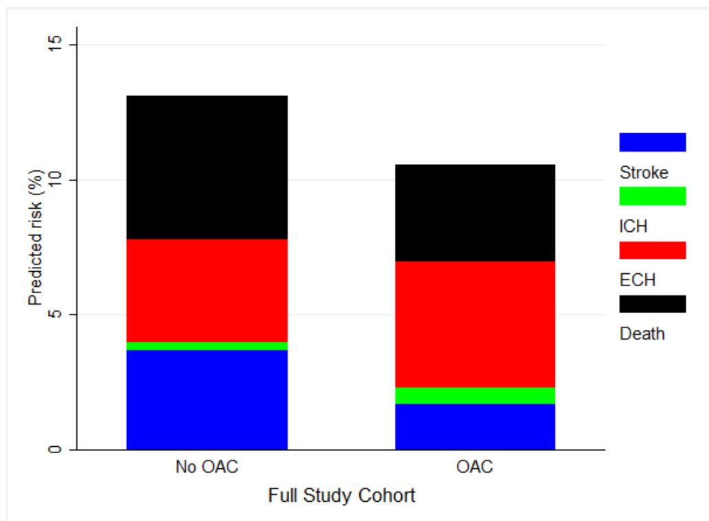
Supplemental Figure 8. Average predicted 1-year risks of clinical events – full study cohort, N=15,483
