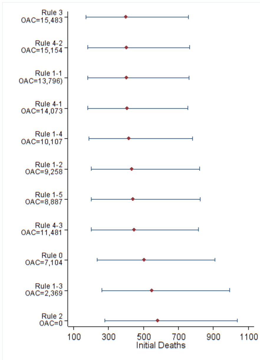
Supplemental Figure 5. Mean and 95% Confidence Interval for Number of Deaths as Competing Event (10,000 runs)
