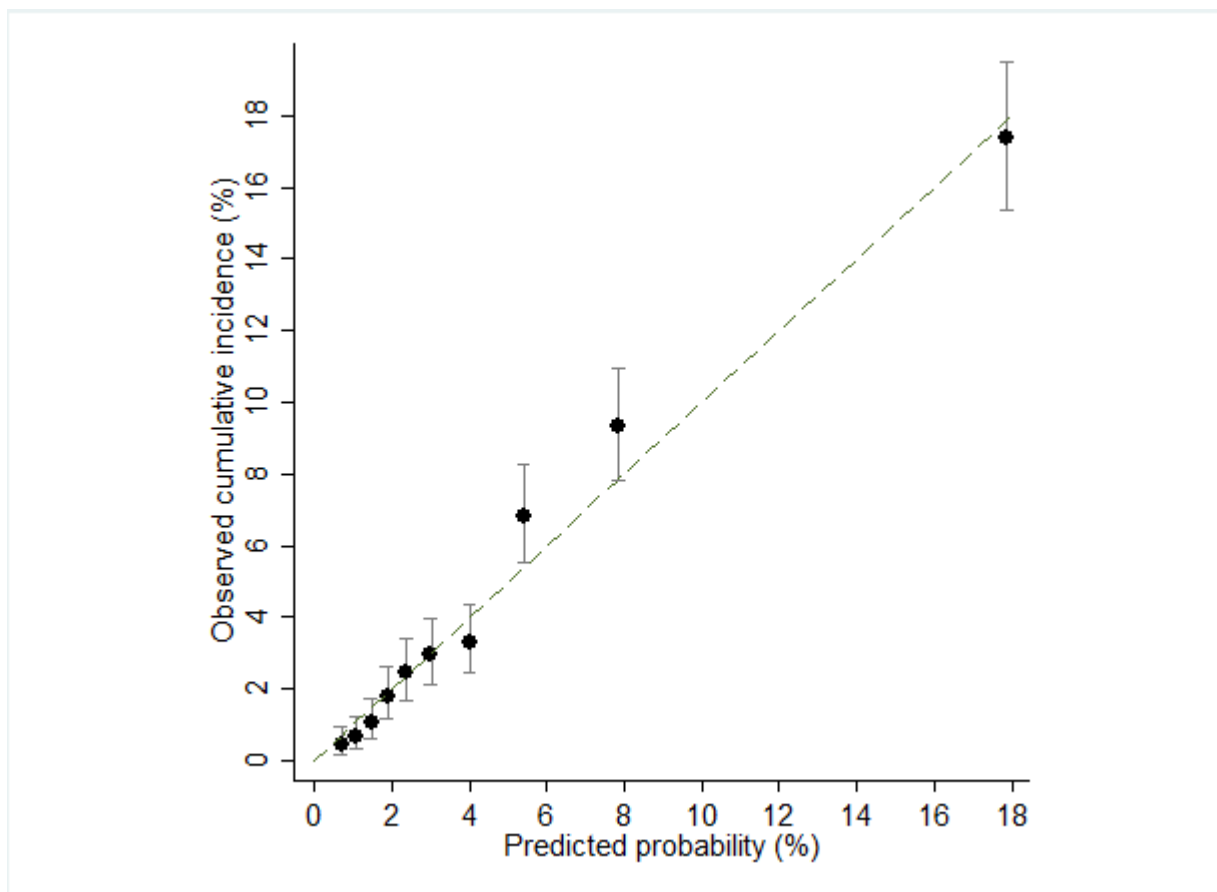
Figure 4.4 Calibration Plot for Death as a First Clinical Event - Full Study Cohort (N=15,483)
