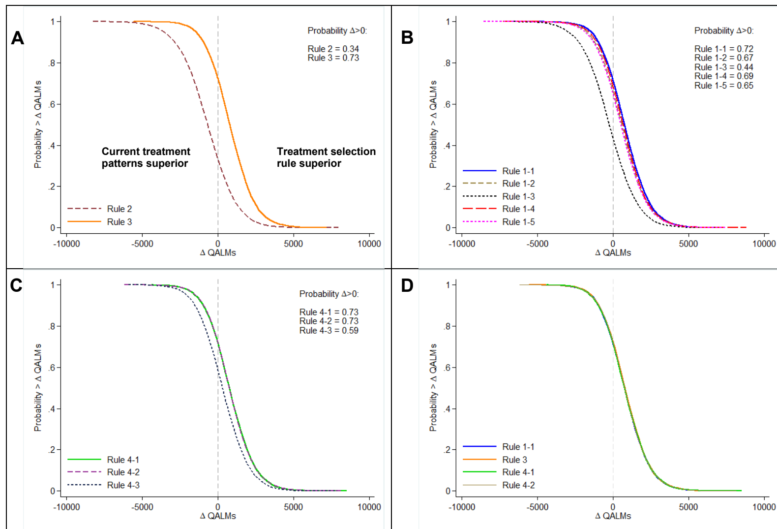
Figure 5.2 Complement Cumulative Distribution Function of QALMs Gained vs. Current Treatment Patterns
