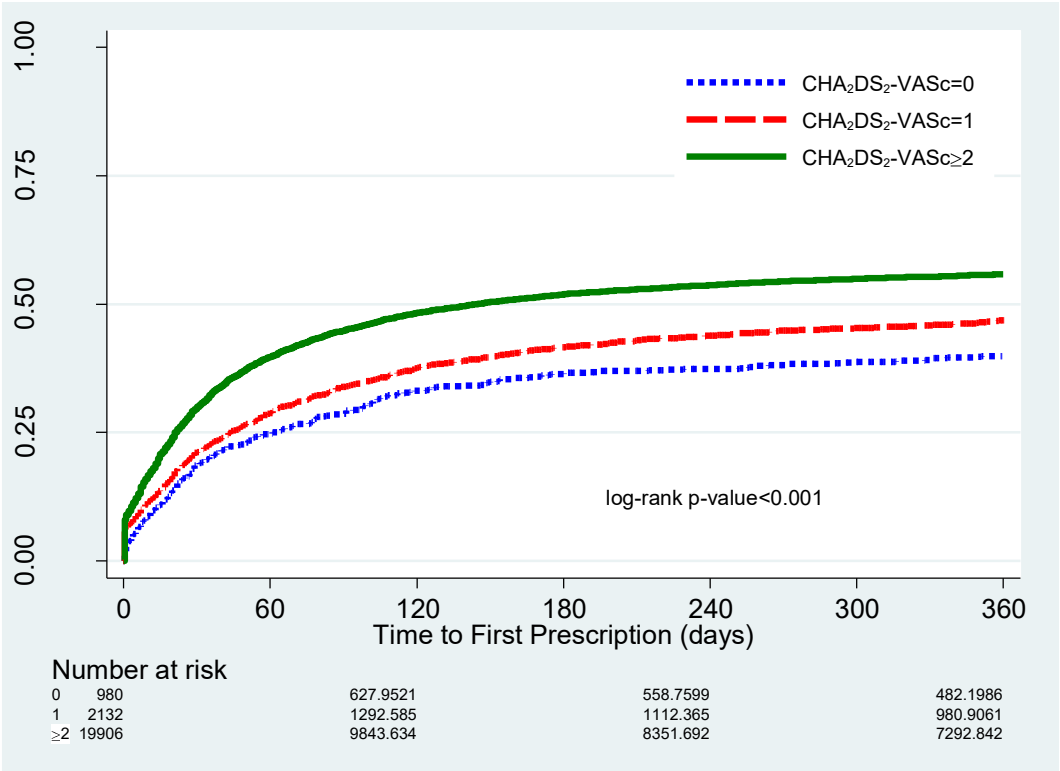
Supplemental Figure 1. Product-limit estimate of the cumulative incidence of first OAC prescription by CHA 2 DS 2 -VASc risk score. Death is treated as a competing event.
