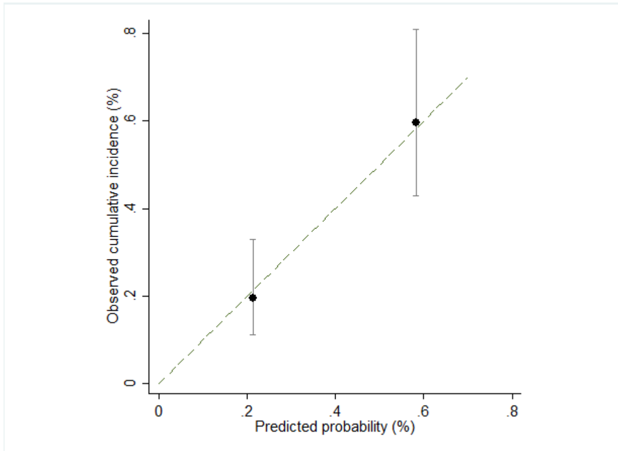
Figure 4.2 Calibration Plot for Intracranial Hemorrhage as a First Clinical Event - Full Study Cohort (N=15,483)
