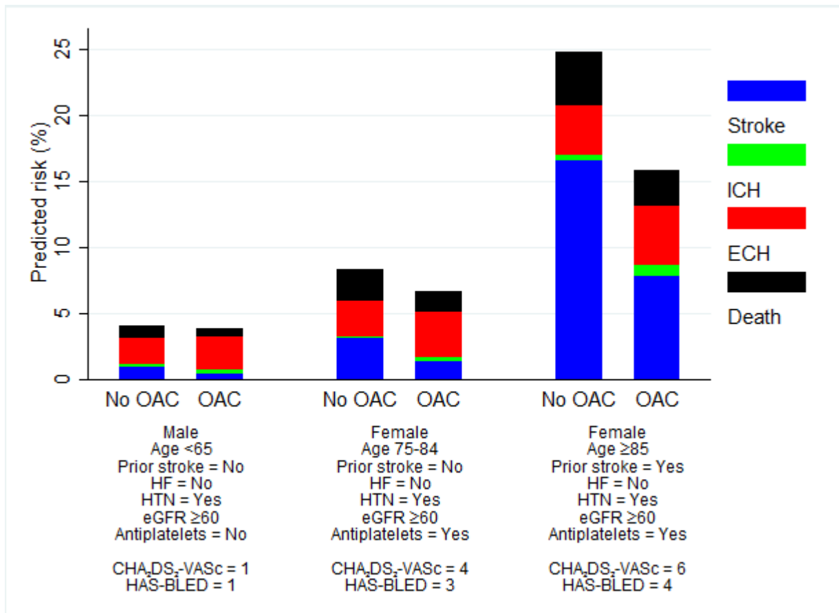
Figure 4.5 Predicted 1-year Risks of Competing First Clinical Events for Patients at Varying Stroke Risk
