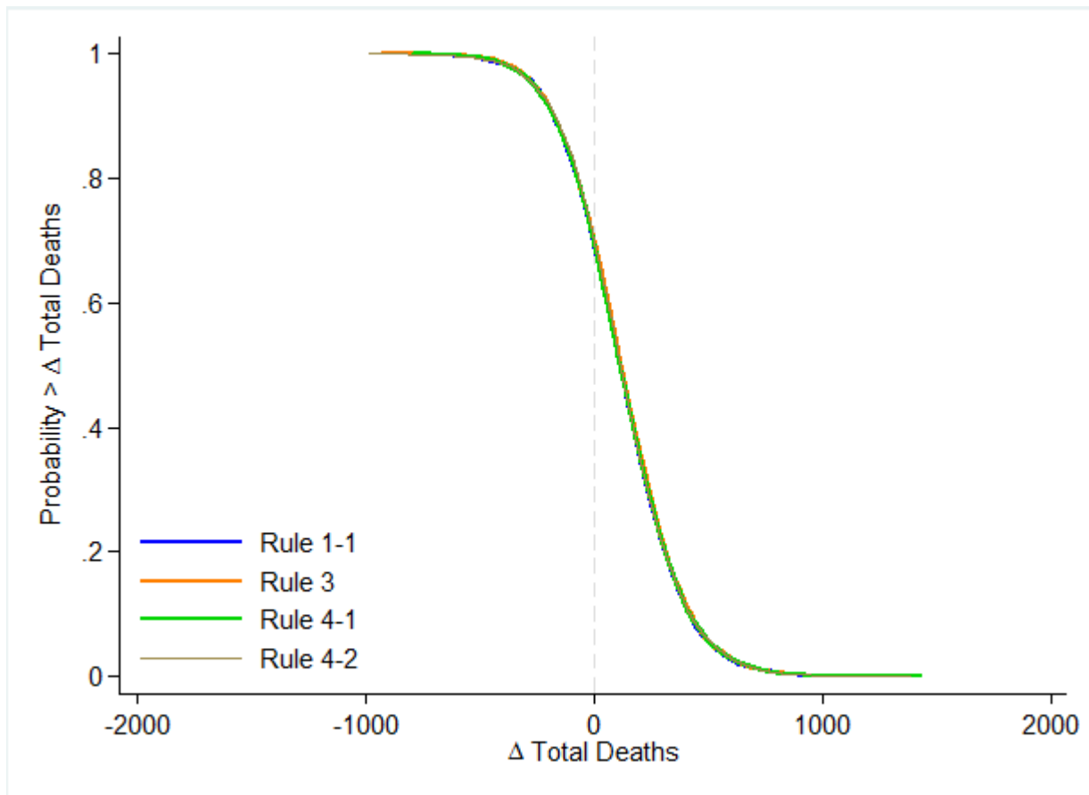
Supplemental Figure 9. Complement Cumulative Distribution Plot of Total Deaths Avoided vs. Current Treatment Patterns for Four Superior Treatment Selection Rules
