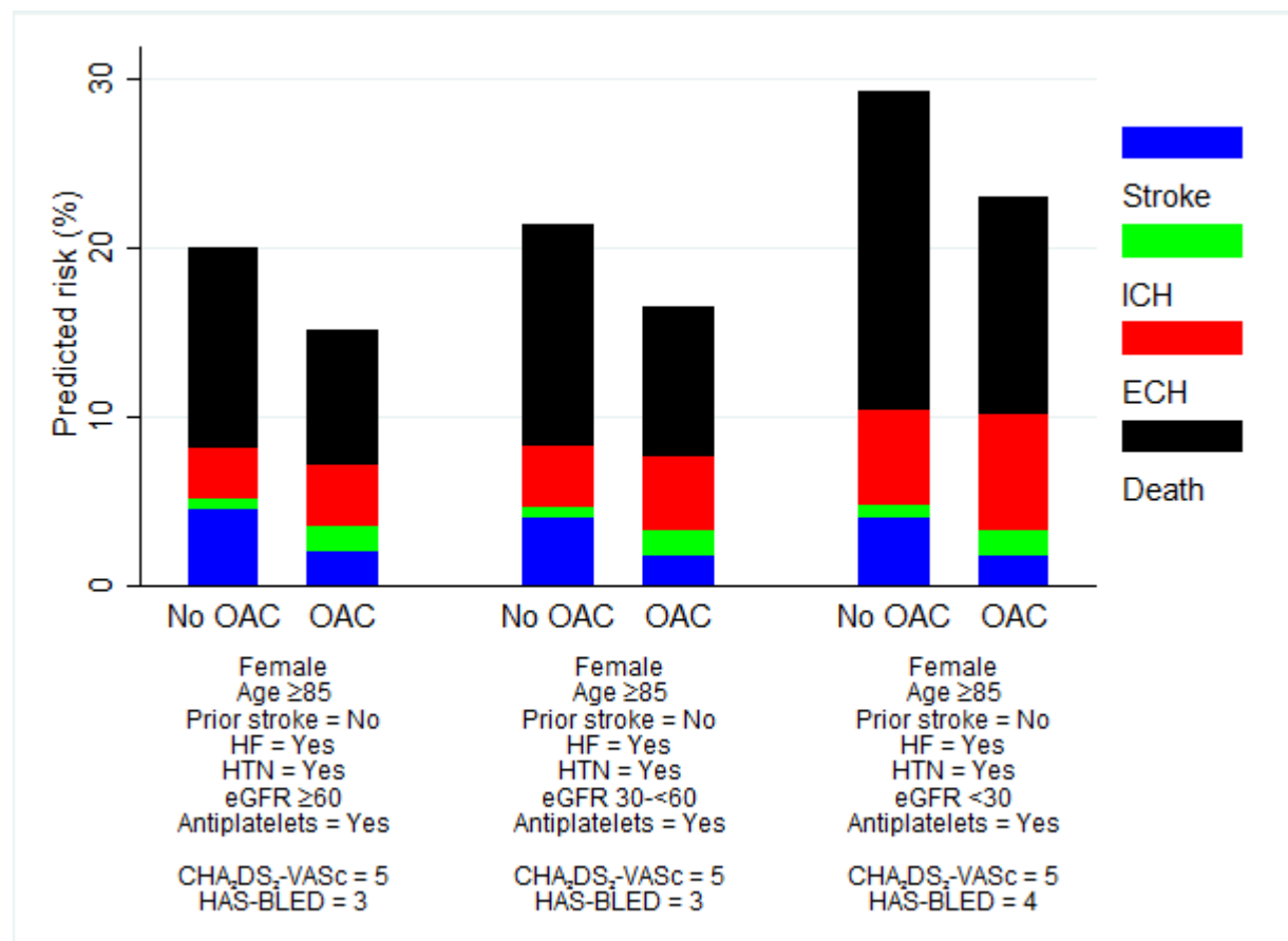
Supplemental Figure 9. Predicted 1-year risks of clinical events for patients at moderate stroke risk with none, moderate, and severe kidney dysfunction
