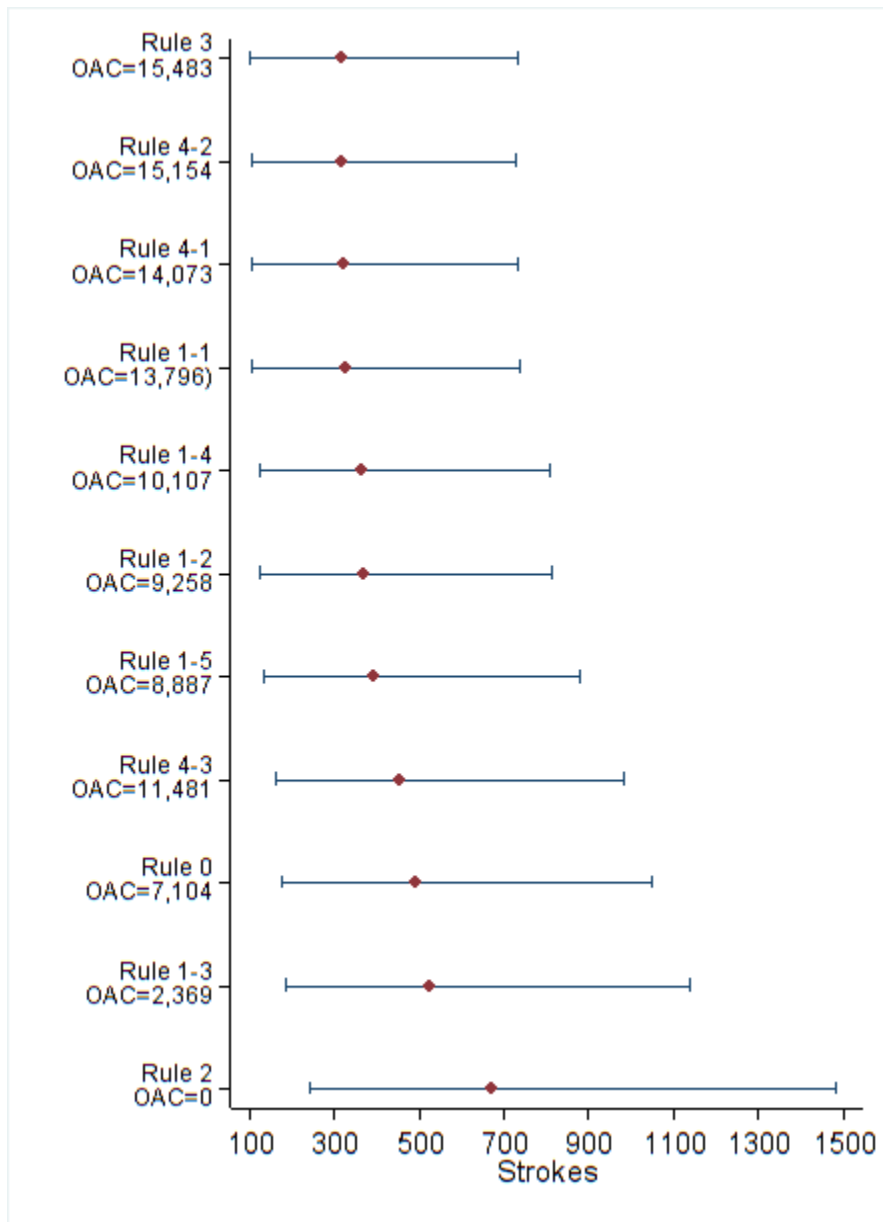
Supplemental Figure 2. Mean and 95% Confidence Interval for Number of Strokes (10,000 runs)
