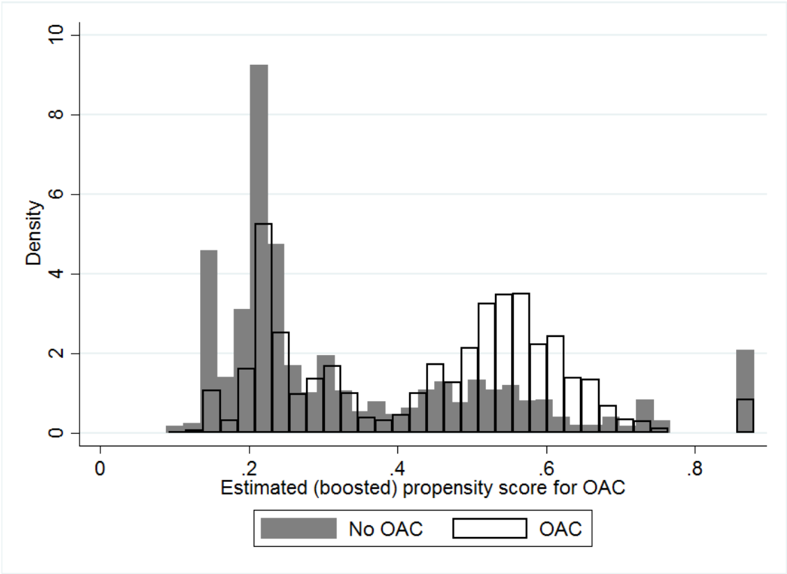
Supplemental Figure 10. Overlapping histograms of estimated propensity scores
