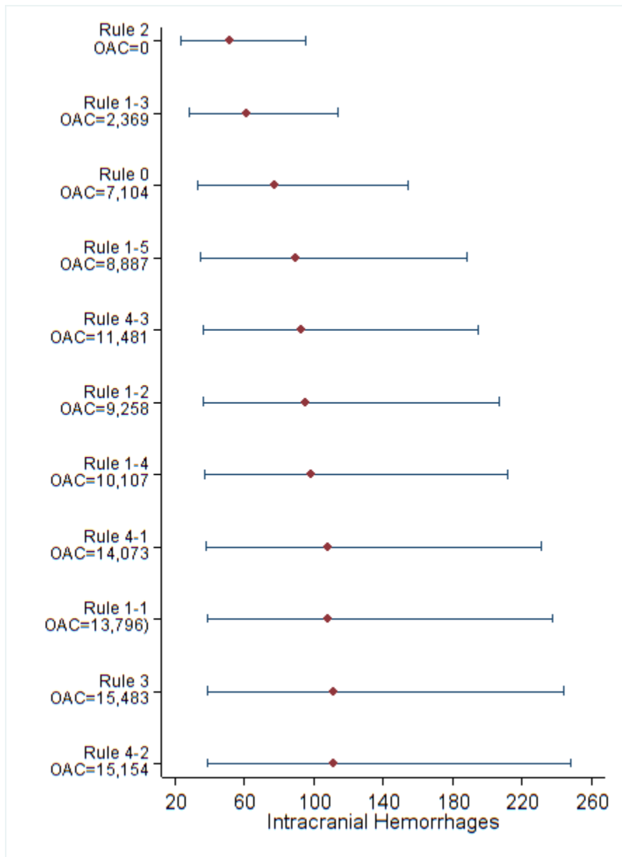
Supplemental Figure 3. Mean and 95% Confidence Interval for Number of Intracranial Hemorrhages (10,000 runs)
