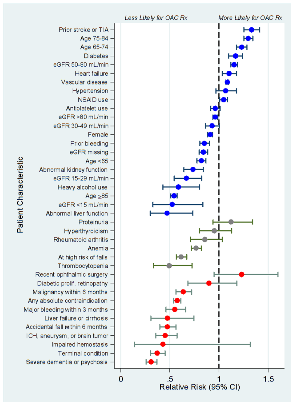
Figure 3.4 Relative Risk (95% CI) of OAC vs. No OAC within 90 days of AF Diagnosis - Patients Diagnosed with NVAF Between 2010 and 2014
