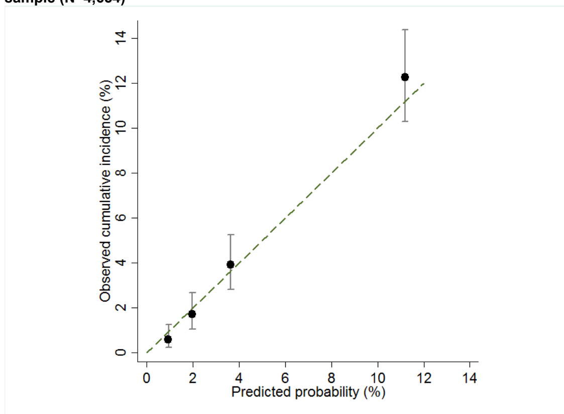
Supplemental Figure 7. Calibration plot for death as a first clinical event – validation sample (N=4,654)
