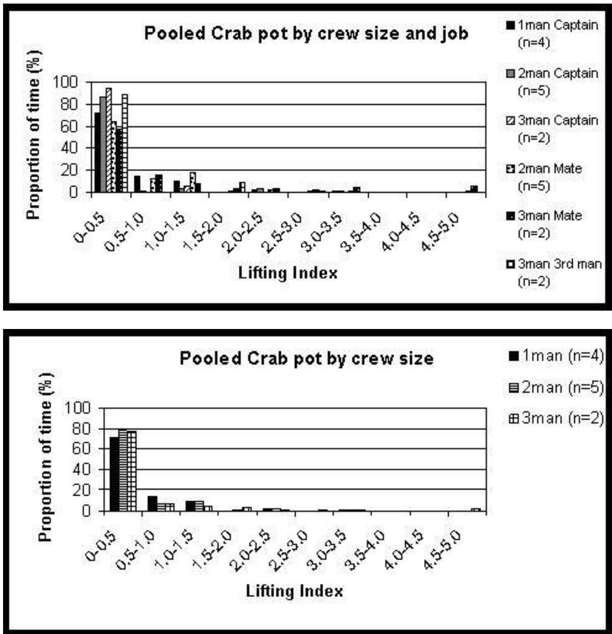
Figure 8.8. Histogram of NIOSH Lifting Index for crab pot fishing pooled for crew size by job and by crew size using Continuous Assessment of Back Stress (CABS) method
