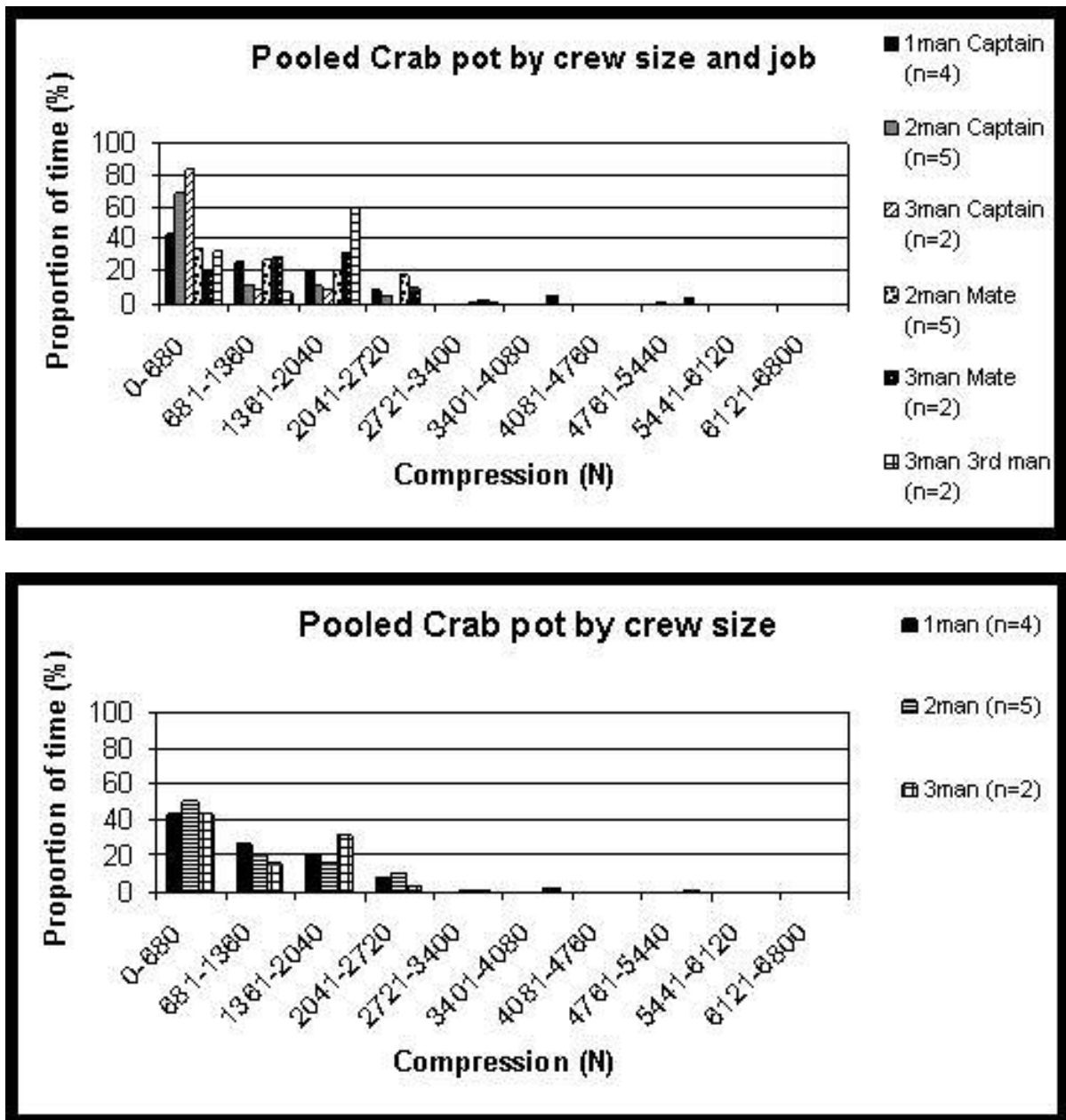
Figure 8.7. Histogram of 3DSSPP Compression for crab pot fishing pooled for crew size by job and by crew size using Continuous Assessment of Back Stress (CABS) method
