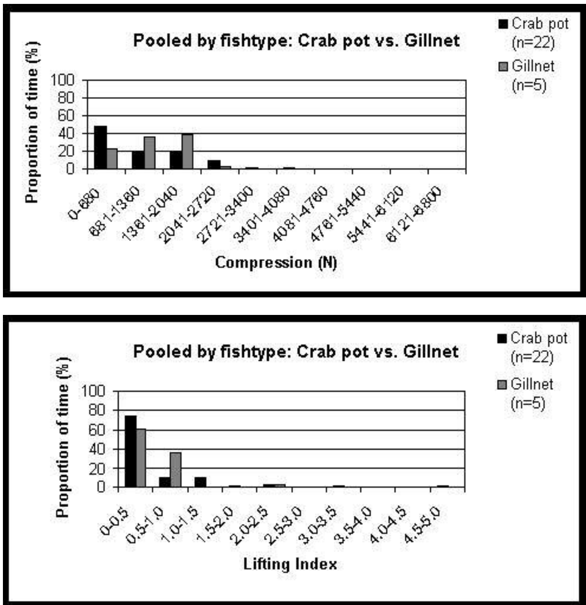
Figure 8.9. Histogram of 3DSSPP Compression and NIOSH Lifting Index pooled across fishing type crab pot and gillnet using Continuous Assessment of Back Stress (CABS) method
