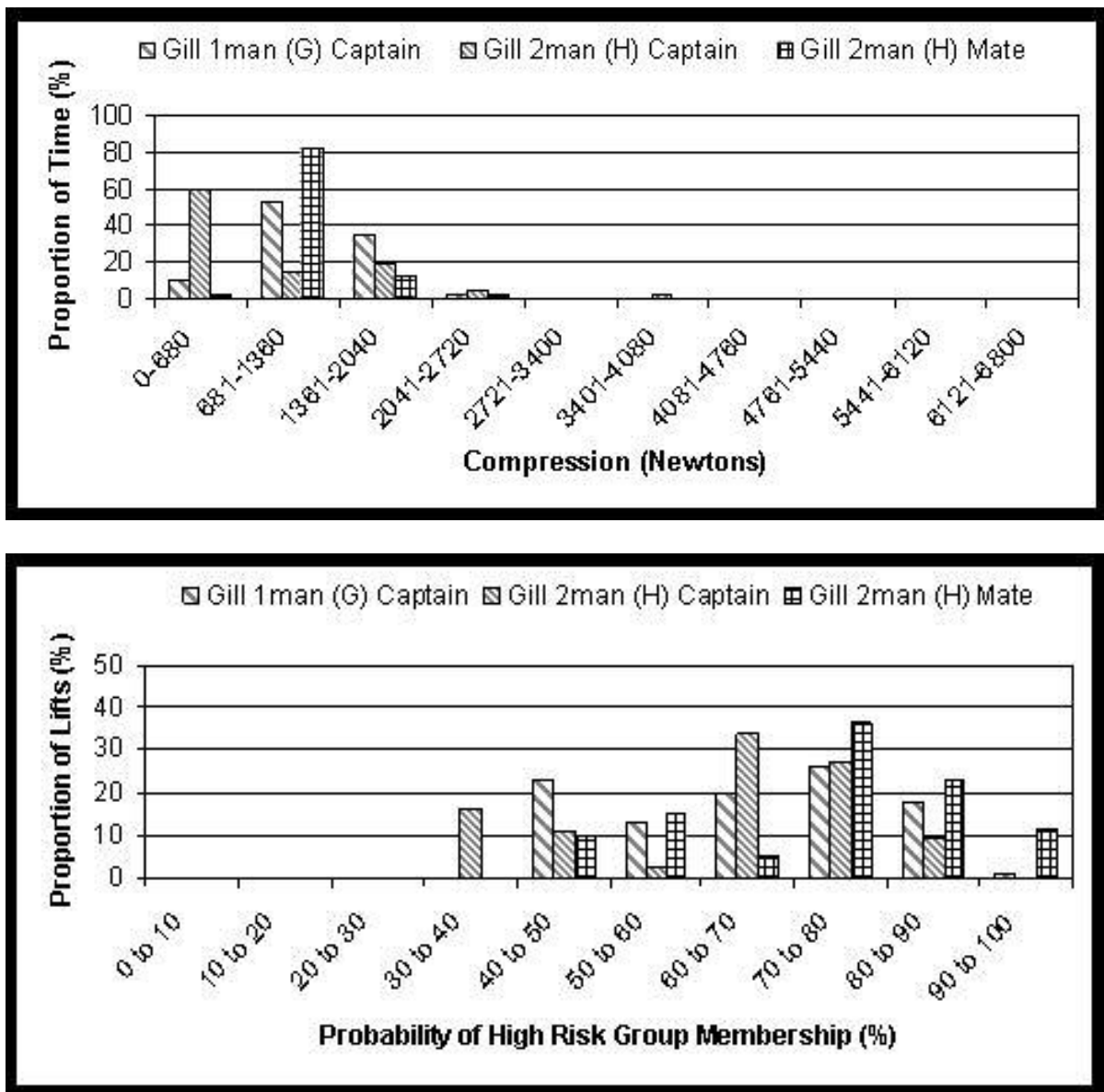
Figure 4.4. Histogram of lumbar spine compression (Newtons), Probability of High Risk Group Membership, and Lifting Index for gillnet fishing captains and mates across different crew sizes, Continuous Assessment of Back Stress method (CABS)
