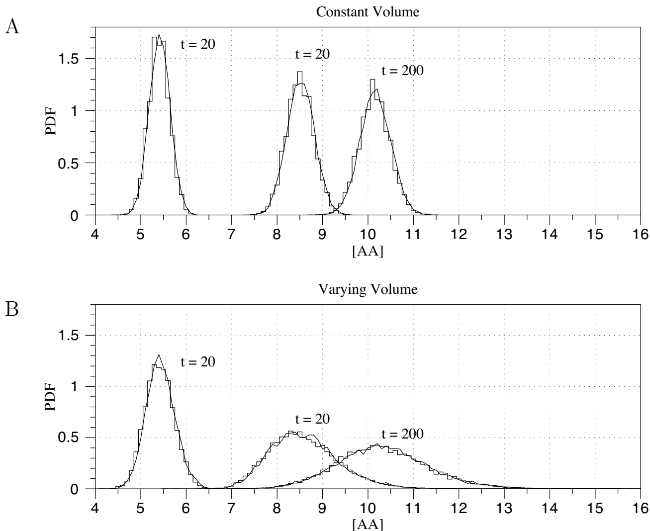
Figure 3 PDFs for the dimer concentration at various times. The staircase plots are the results for the discrete case and the continuous lines are the results for the continuous case. Panel A is for the case of constant volume and Panel B is the varying volume case. The parameter values and initial conditions are the same as in Figs. 2 and 4, for the constant volume case and varying volume case, respectively. Each PDF consists of 10, 000 realizations of the process.
